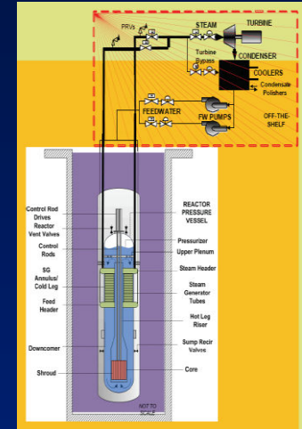
NuScale
