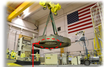
ATR's vessel head being lifted into place after CIC with new top head closure plate installed
